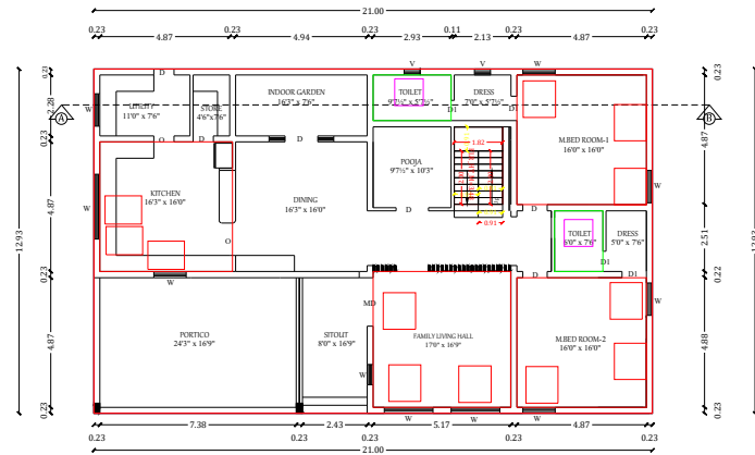
EXISTING GROUND FLOOR PLAN
