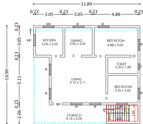
PRO.GROUND FLOOR PLAN
