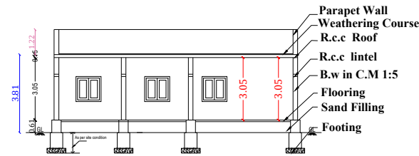
SECTION A - B
