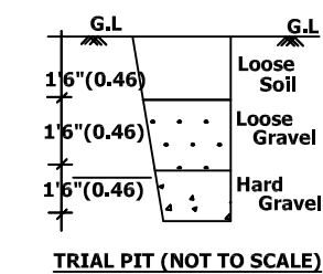
TRIAL PIT (NOT TO SCALE)
