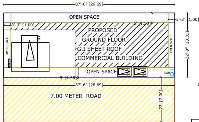
SUPER IMPOSED SITE PLAN
