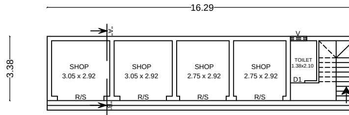
PRO.GROUND FLOOR PLAN
