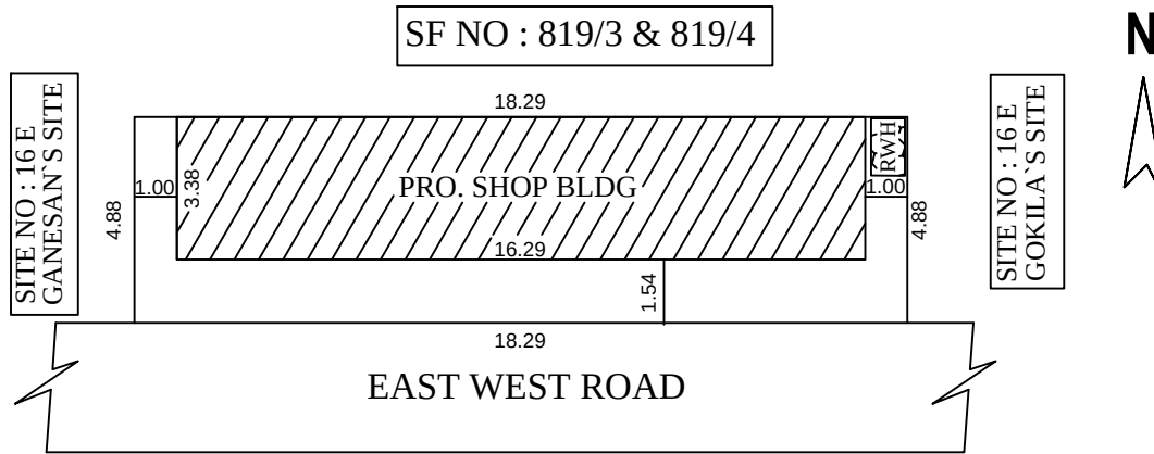
SITE PLAN
