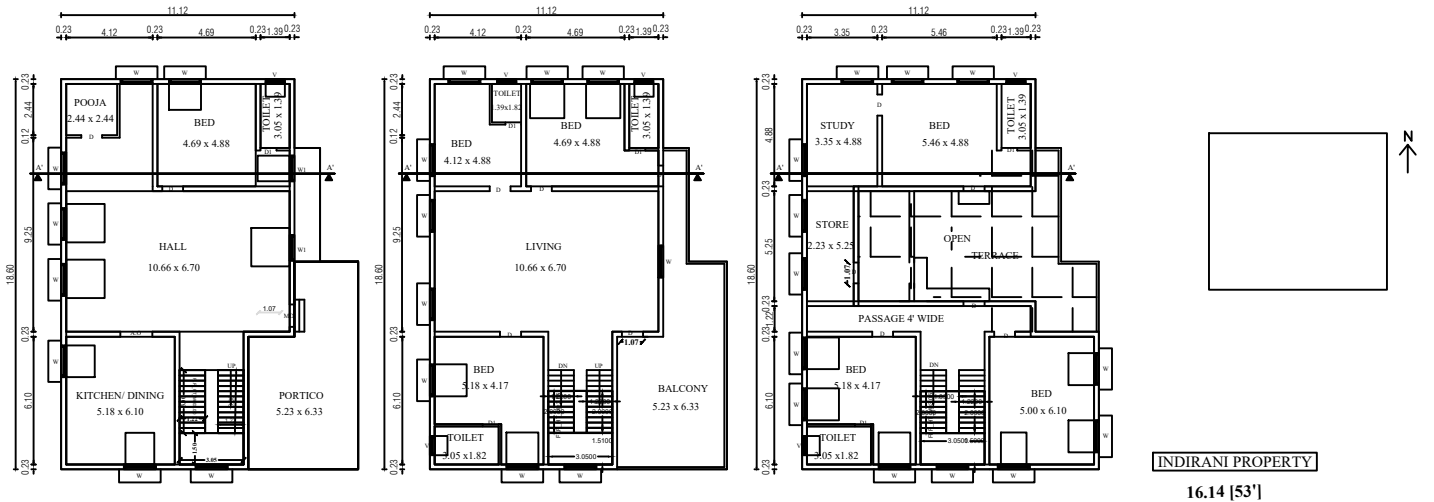
OR PLAN
