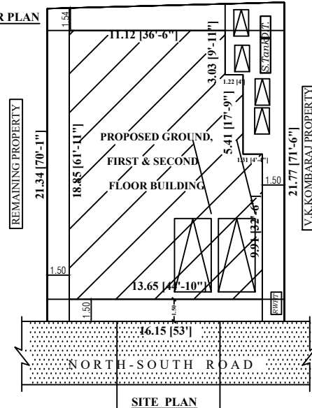
SITE PLAN
