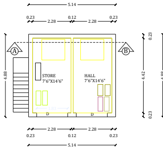
ADD.GROUND FLOOR PLAN
