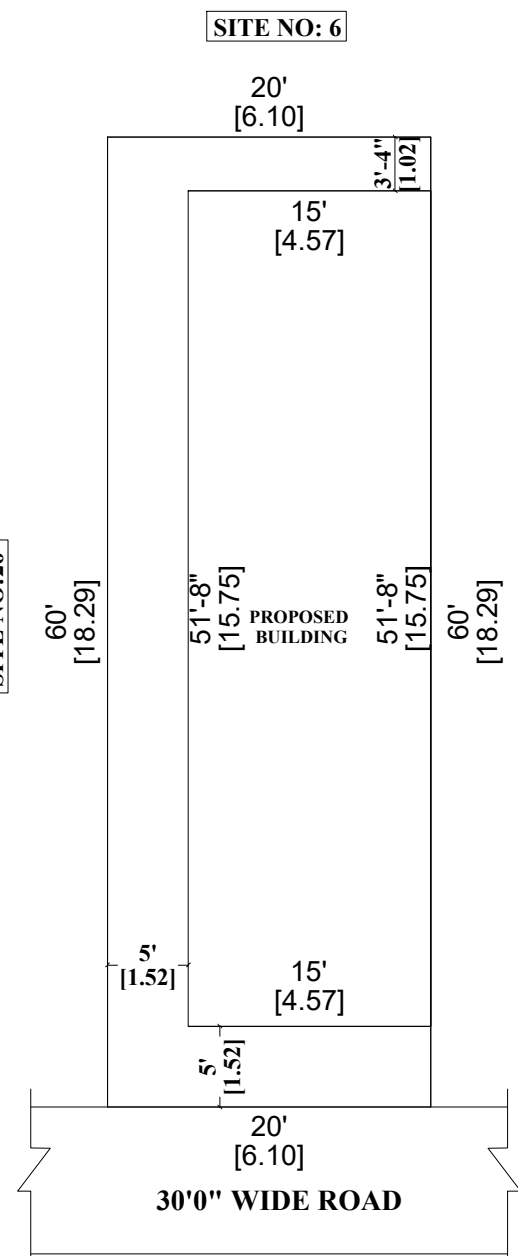
Site Plan
