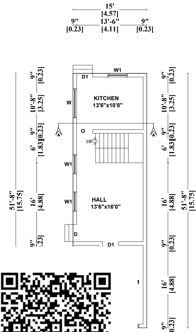
Plan
