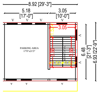
SILT FLOOR PLAN
