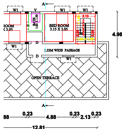
FIRST FLOOR PLAN (Proposed Building)
