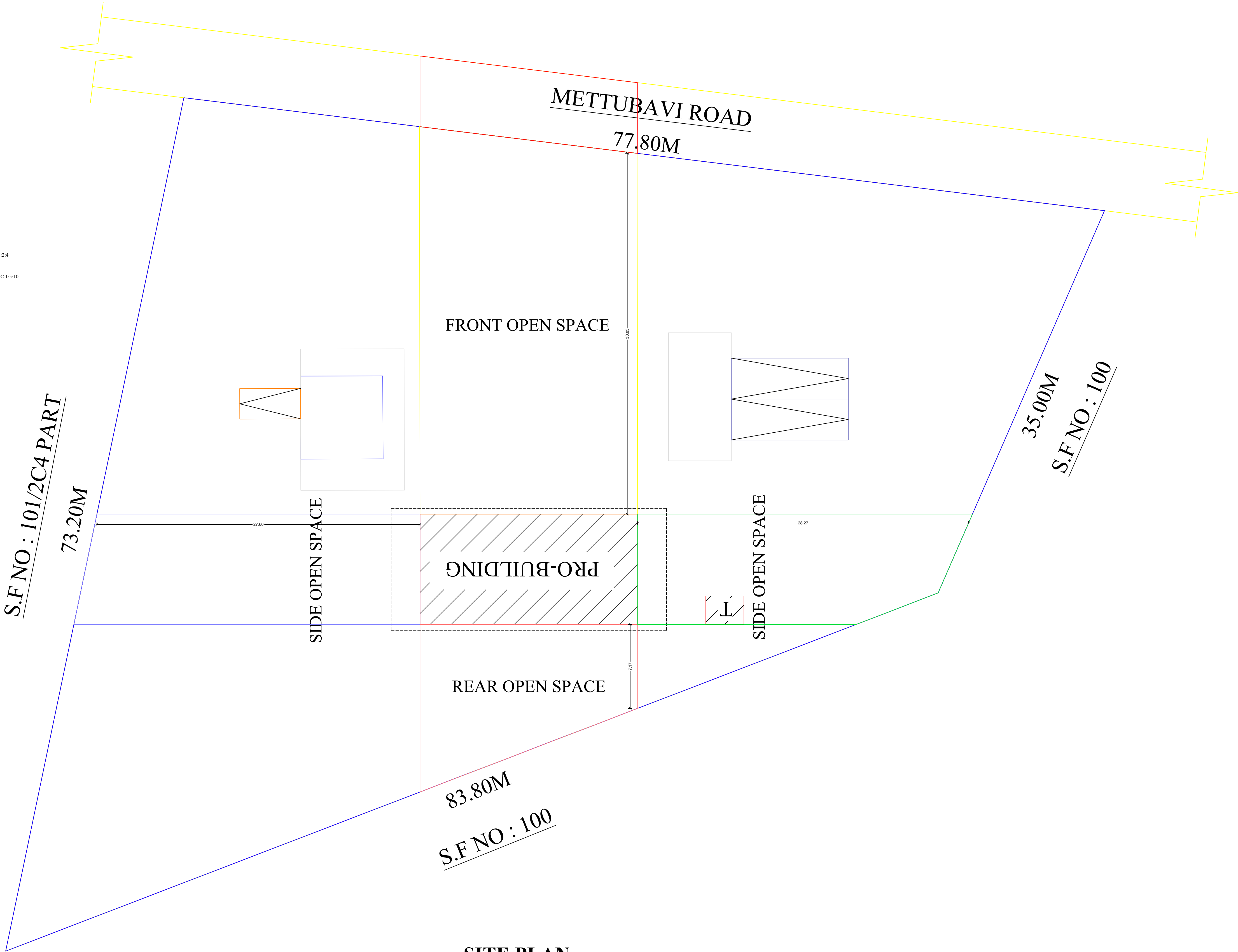
SITE PLAN
