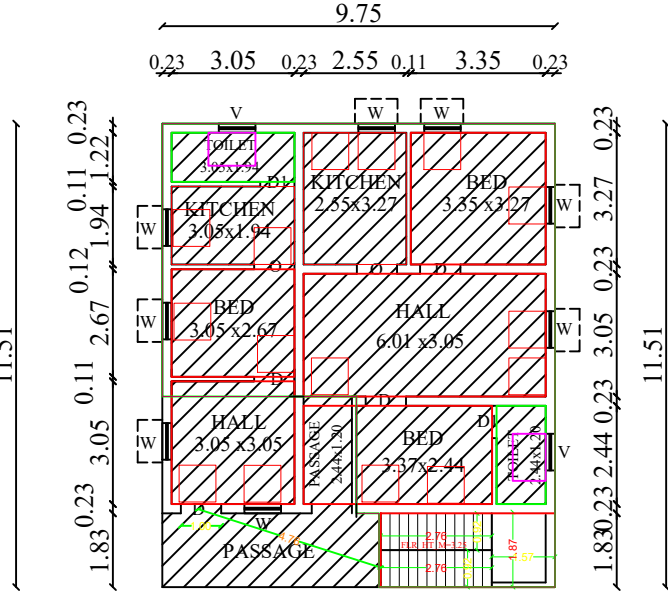
PLAN for Existing First Floor
