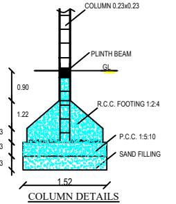
COLUMN DETAILS
