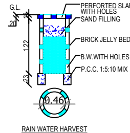
RAIN WATER HARVEST
