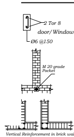
Vertical Reinforcement in brick walls
