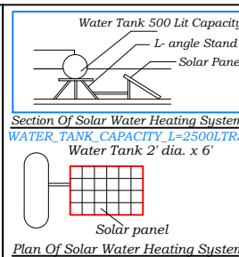
Plan Of Solar Water Heating System
