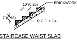
STAIRCASE WAIST SLAB
