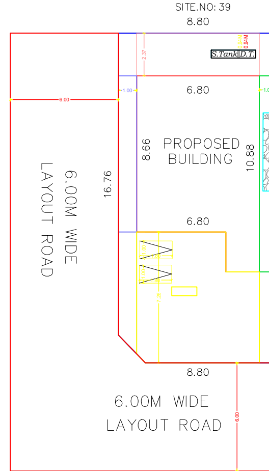
SITE PLAN
