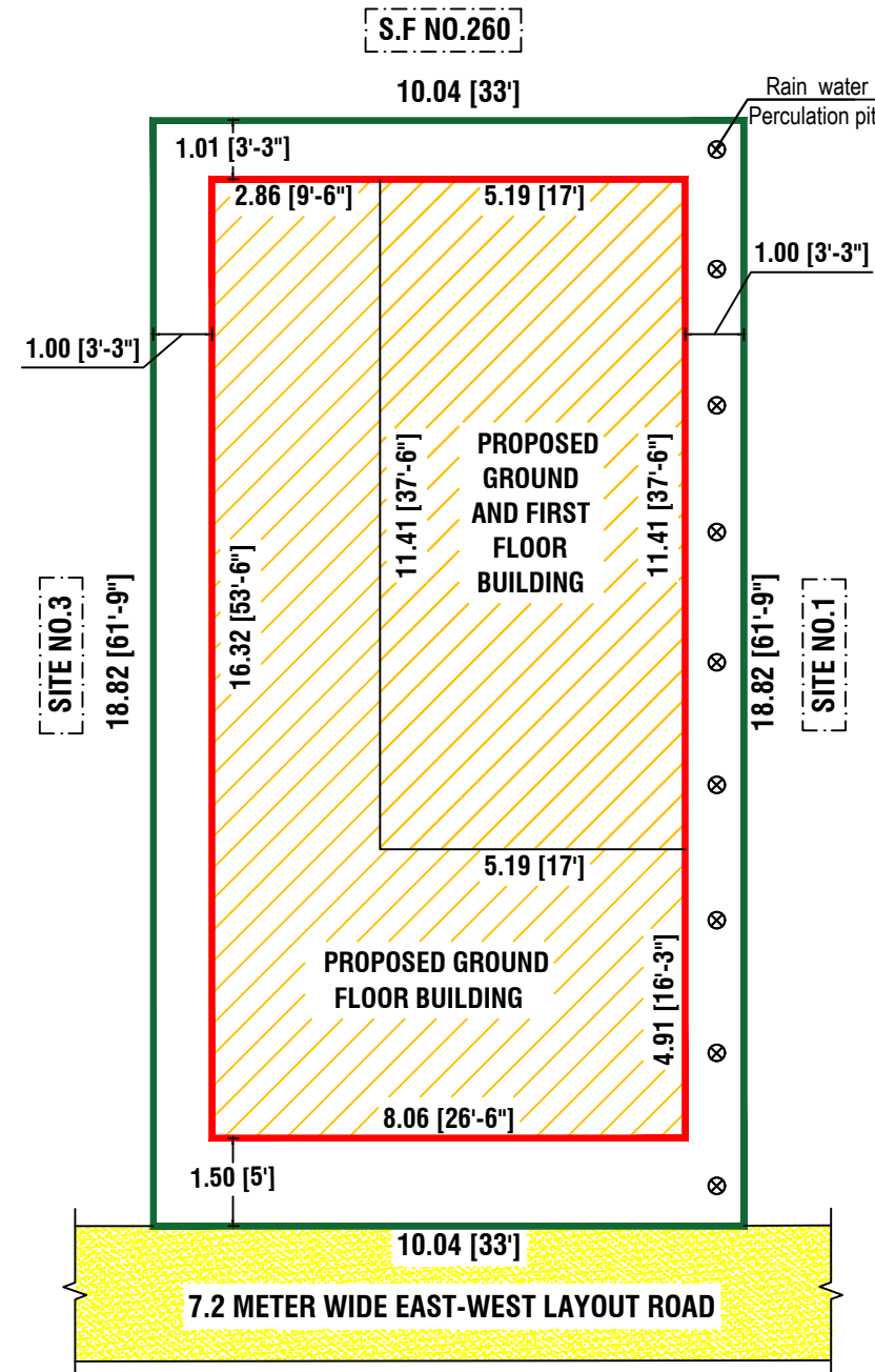
SITE PLAN
