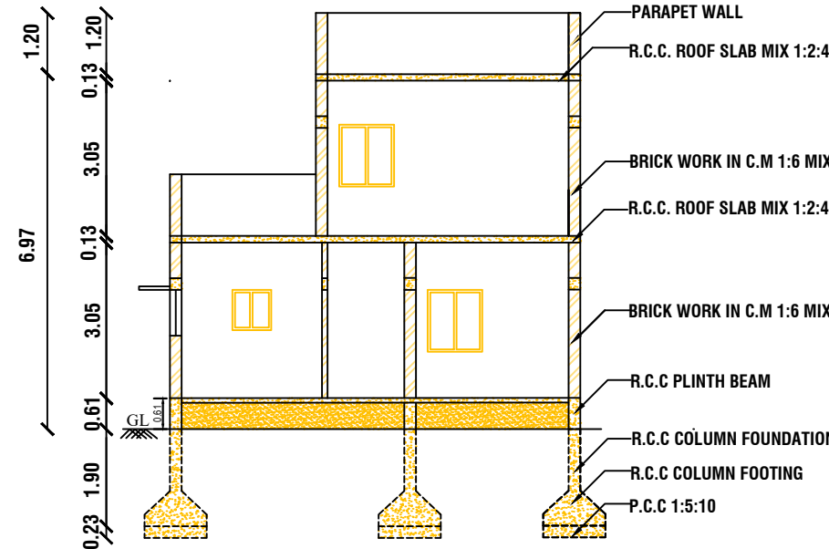
CROSS SECTION AT A-A
