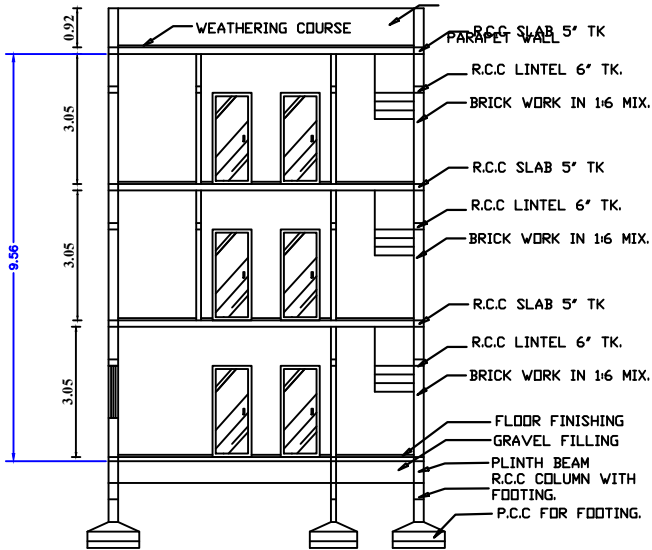
CROSS SECTION AT A-A
