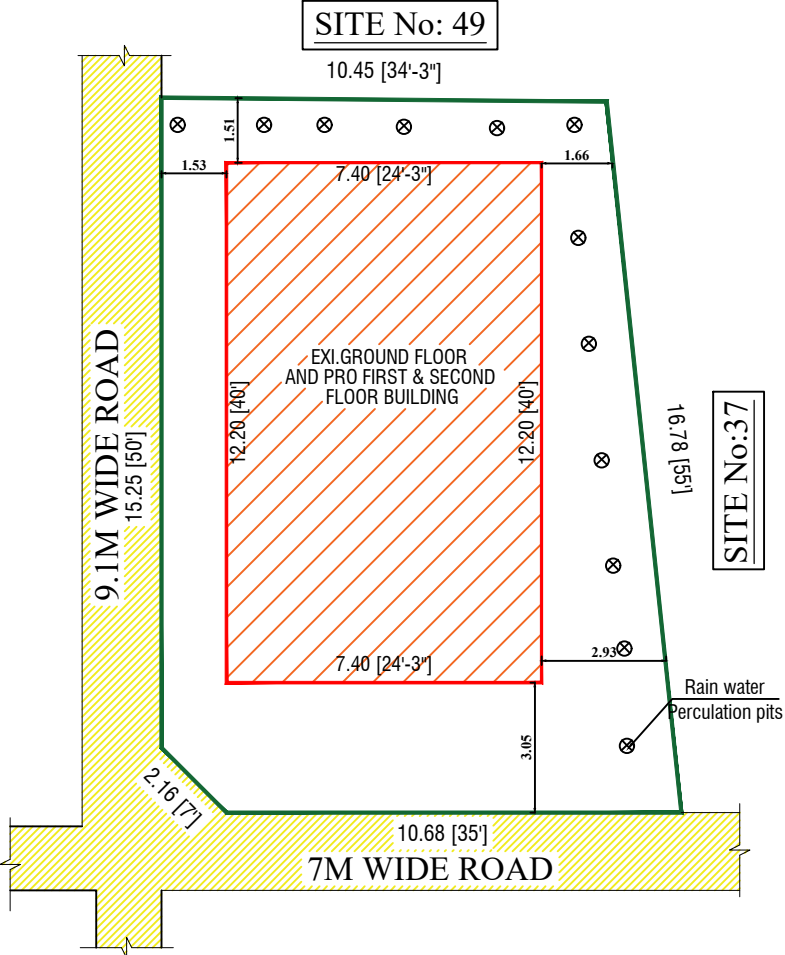
SITE PLAN
