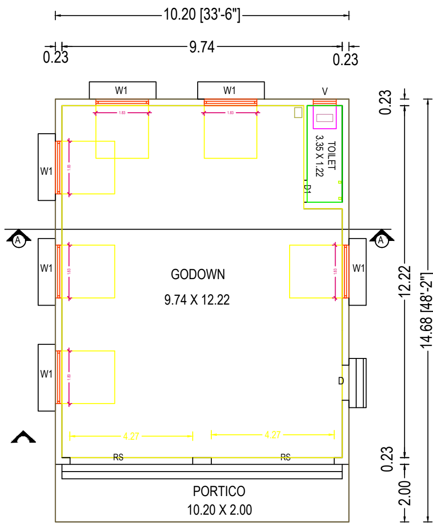
D FLOOR PLAN
