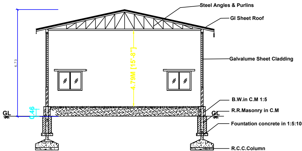
CROSS SECTION ON A-A'
