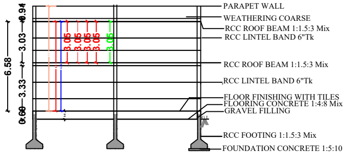
SECTION ON A-A SCALE 1:100
