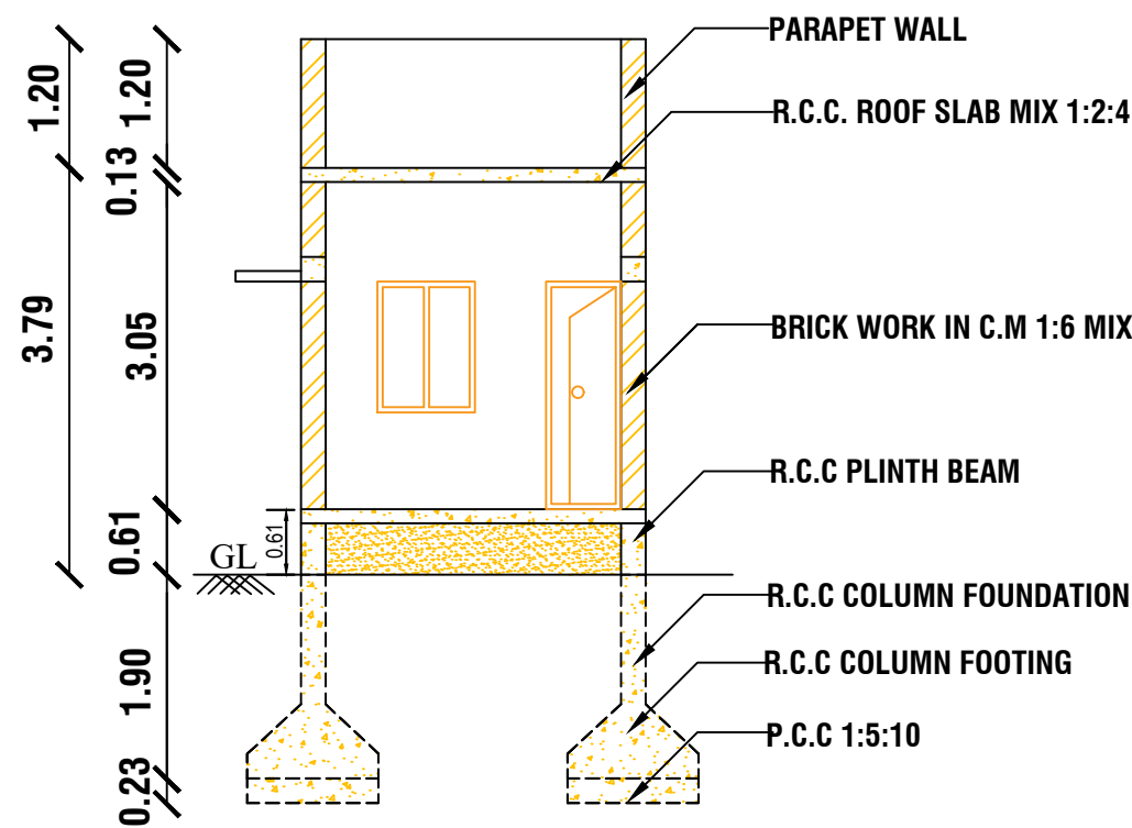
CROSS SECTION AT A-A
