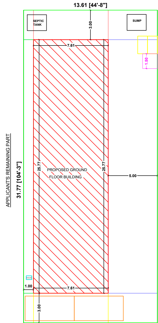
CONCERN SITE PLAN
