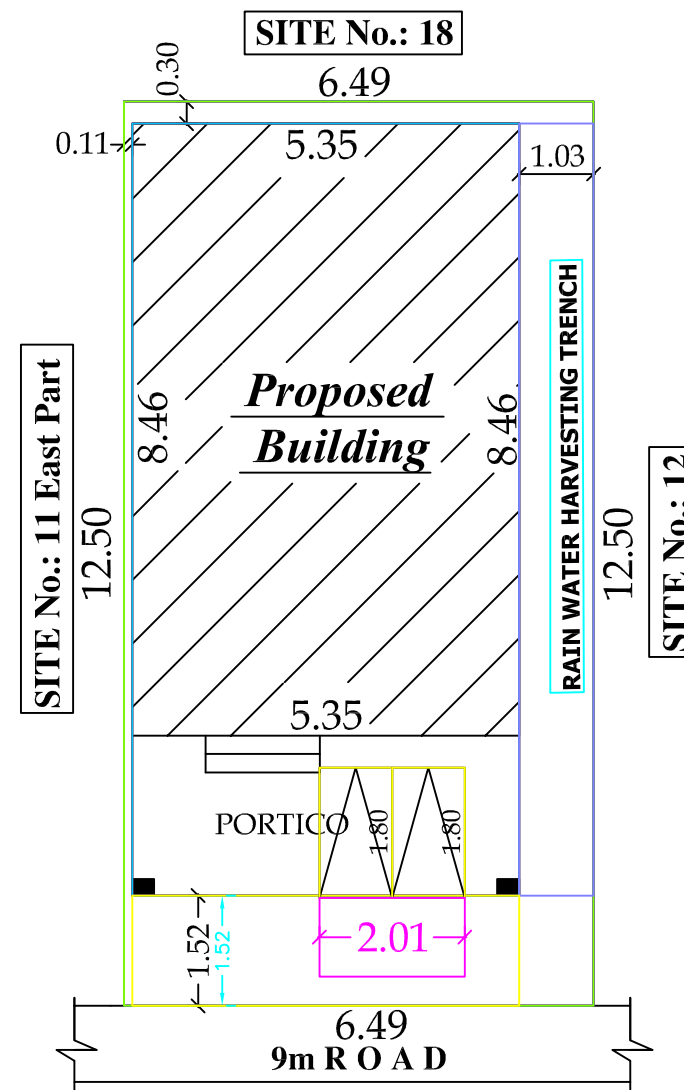
SITE PLAN
