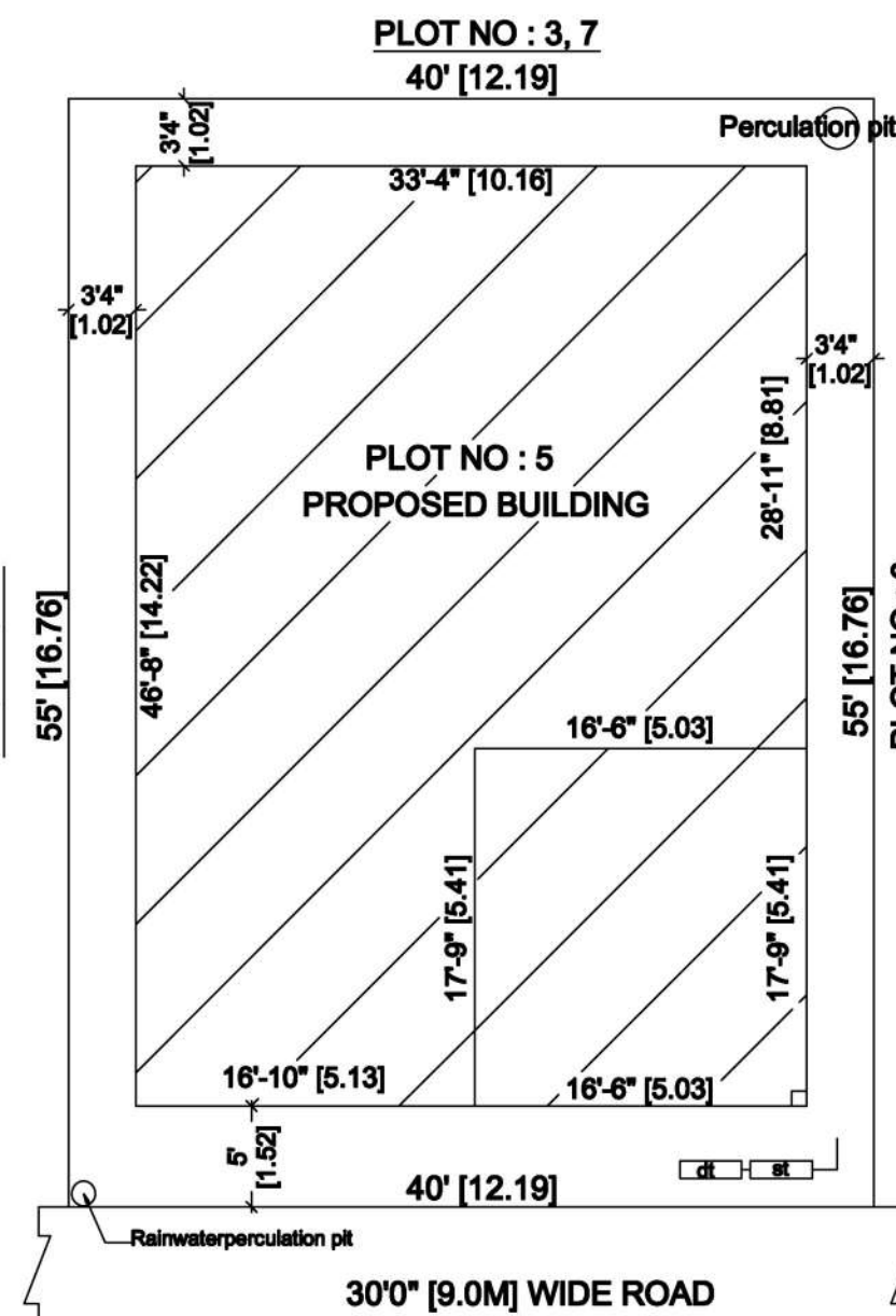
SITE PLAN
