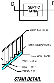
STAIR DETAIL
