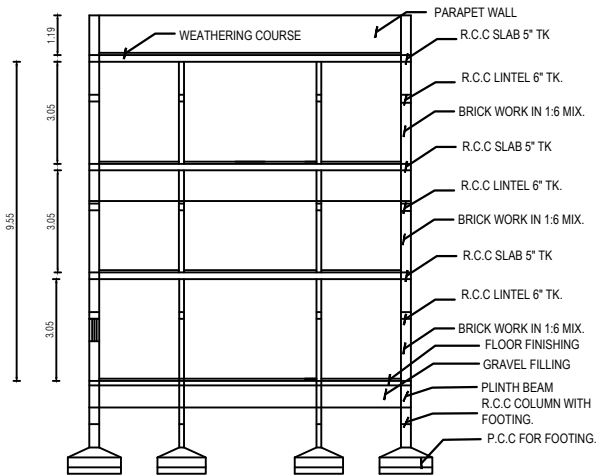
CROSS SECTION AT A-A
