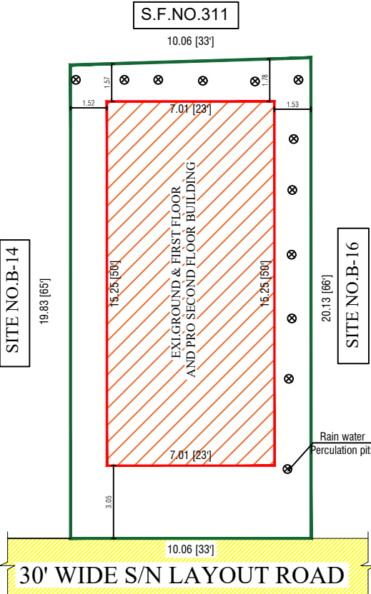
SITE PLAN
