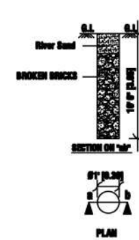
Rain Water Percolation Pit
