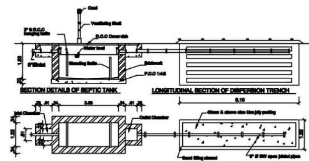
PLAN OF SEPTIC TANK DISPERSION TRENCH (TYP) DETAILS OF SEPTIC TANK - 250 GALLONS
