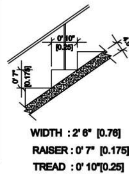
STAIRCASE DETAILS:
