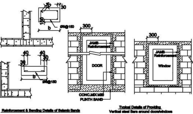
ESSENTIAL INTERNAL ELEMENTS IN BUILDING
