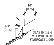
STAIR CASE DETAILS :-
