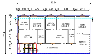
EXISTING GROUND FLOOR PLAN
