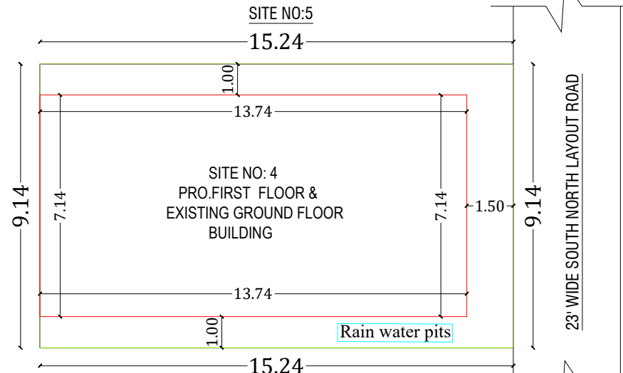
KEY PLAN
