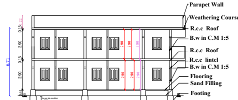
SECTION A - B
