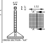
COLUMN DETAILS :-
