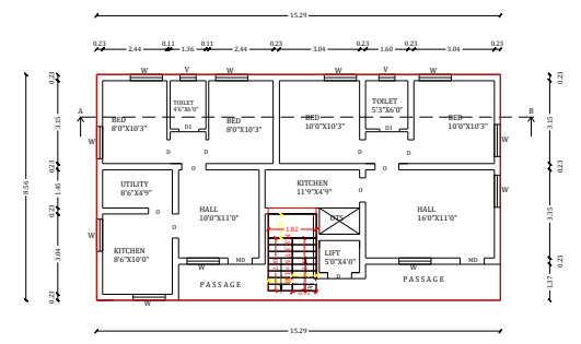
Proposed Second Floor Plan
