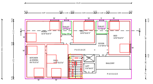
Proposed Third Floor Plan
