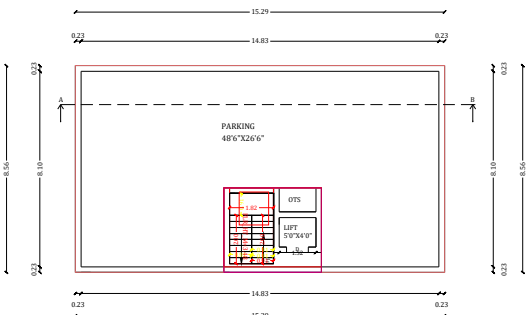
Proposed Stilt Floor Plan
