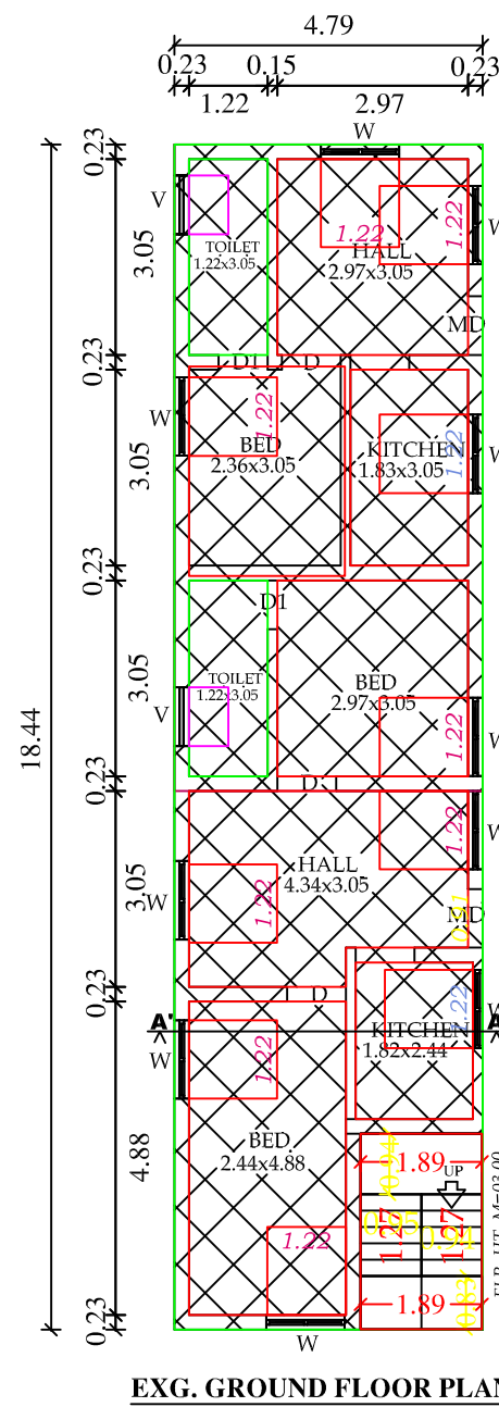
EXG. GROUND FLOOR PLAN
