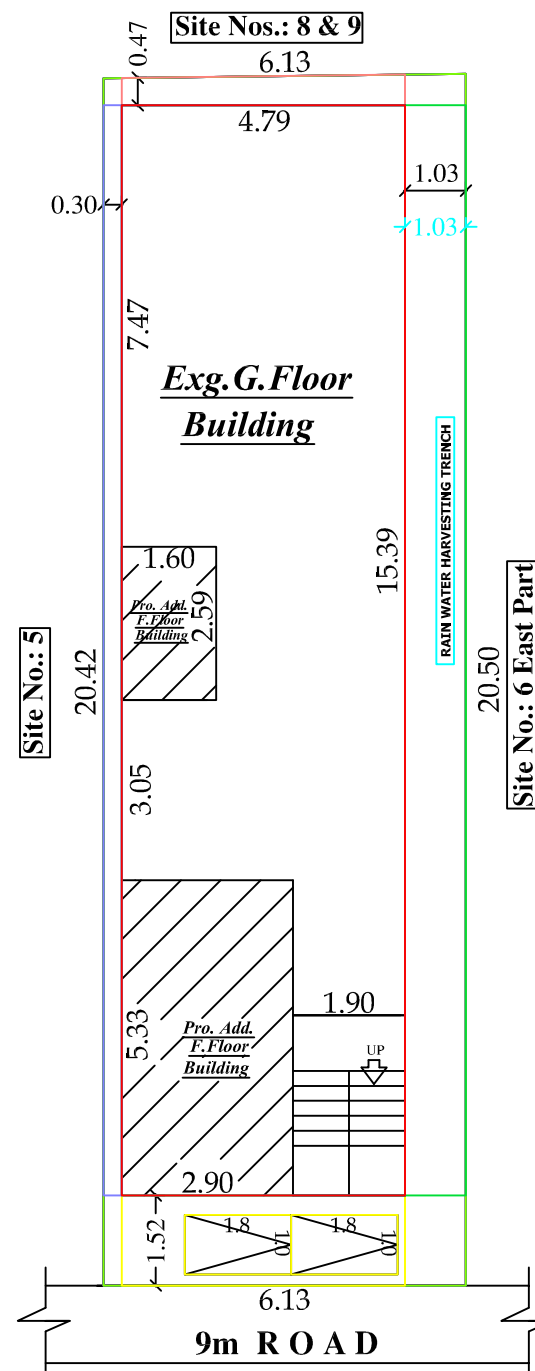
SITE PLAN
