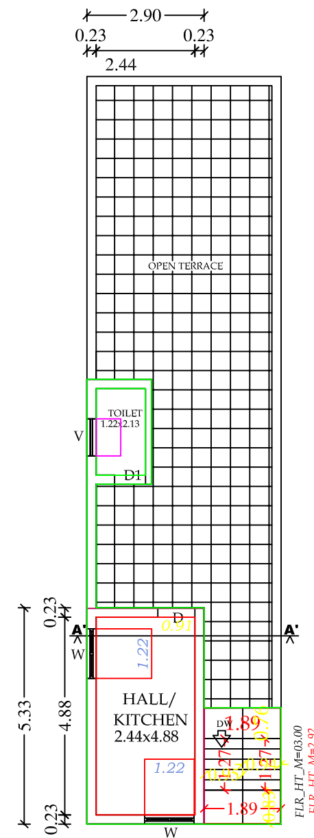
PRO. ADD. FIRST FLOOR PLAN
