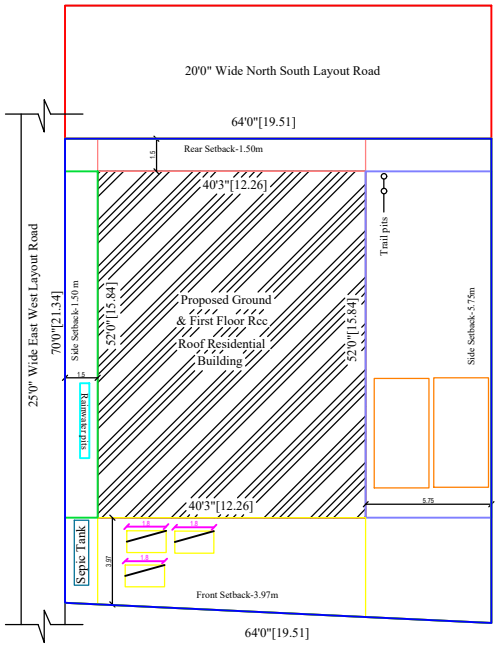
SITE PLAN
