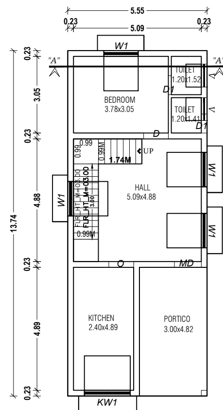
PRO. GROUND FLOOR PLAN
