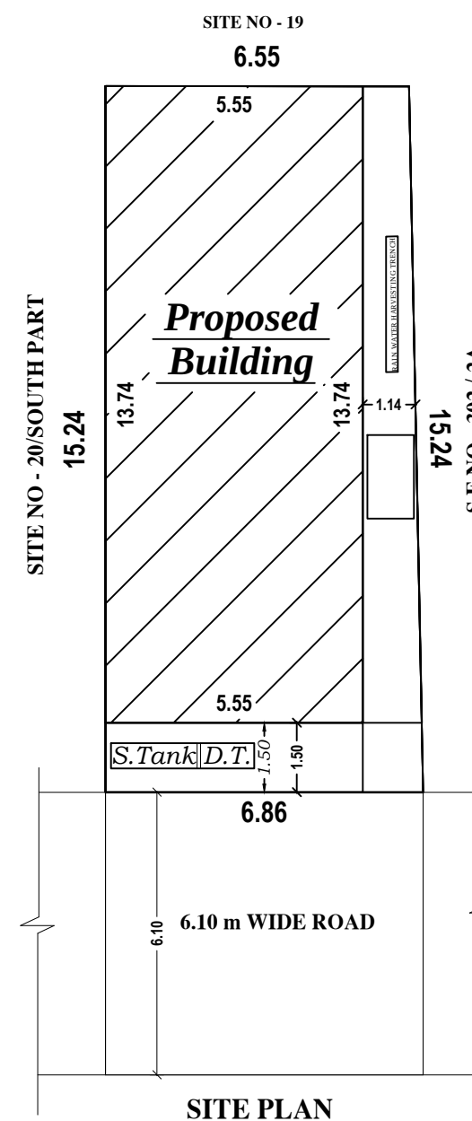
SITE PLAN
