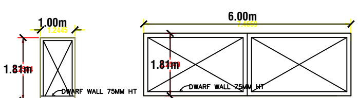
WICKET GATE
