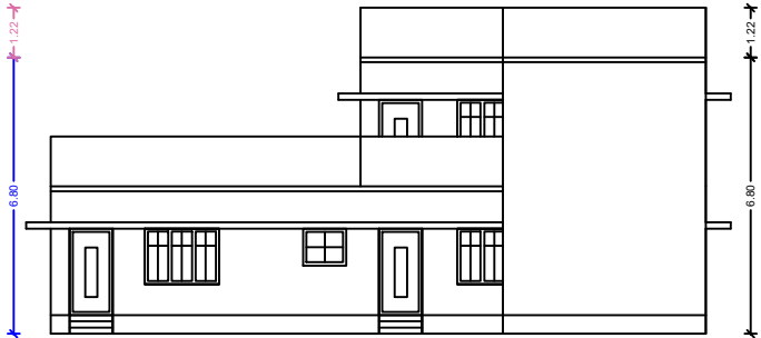
FRONT ELEVATION
