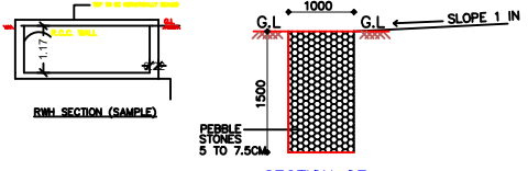
SECTION OF PEBBLE TRENCH SCALE : 1 : = 100
