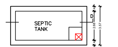
PLAN OF SEPTIC TANK SCALE 1"=2'-0"
