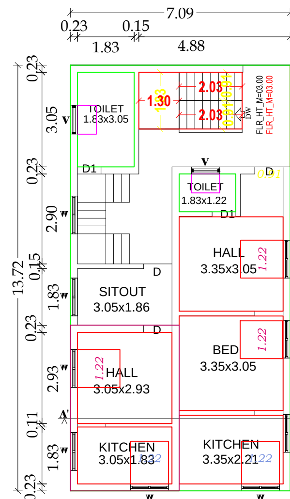
PRO. ADD. FIRST FLOOR PLAN
