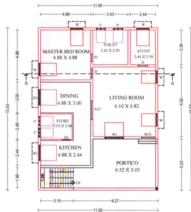
LOOR PLAN
