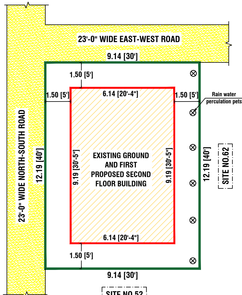
SITE PLAN
