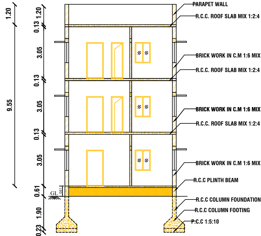
CROSS SECTION AT A-A
