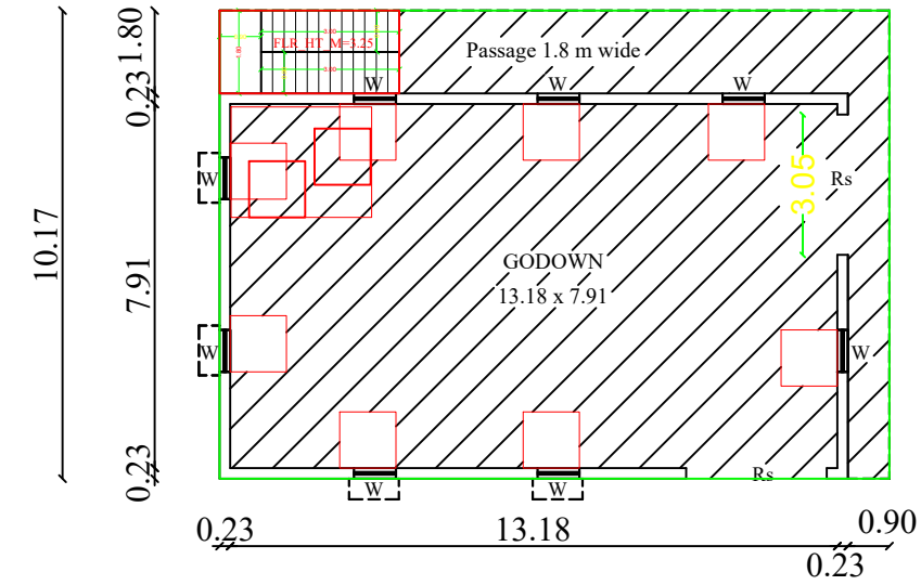
PLAN - Existing Ground Floor
