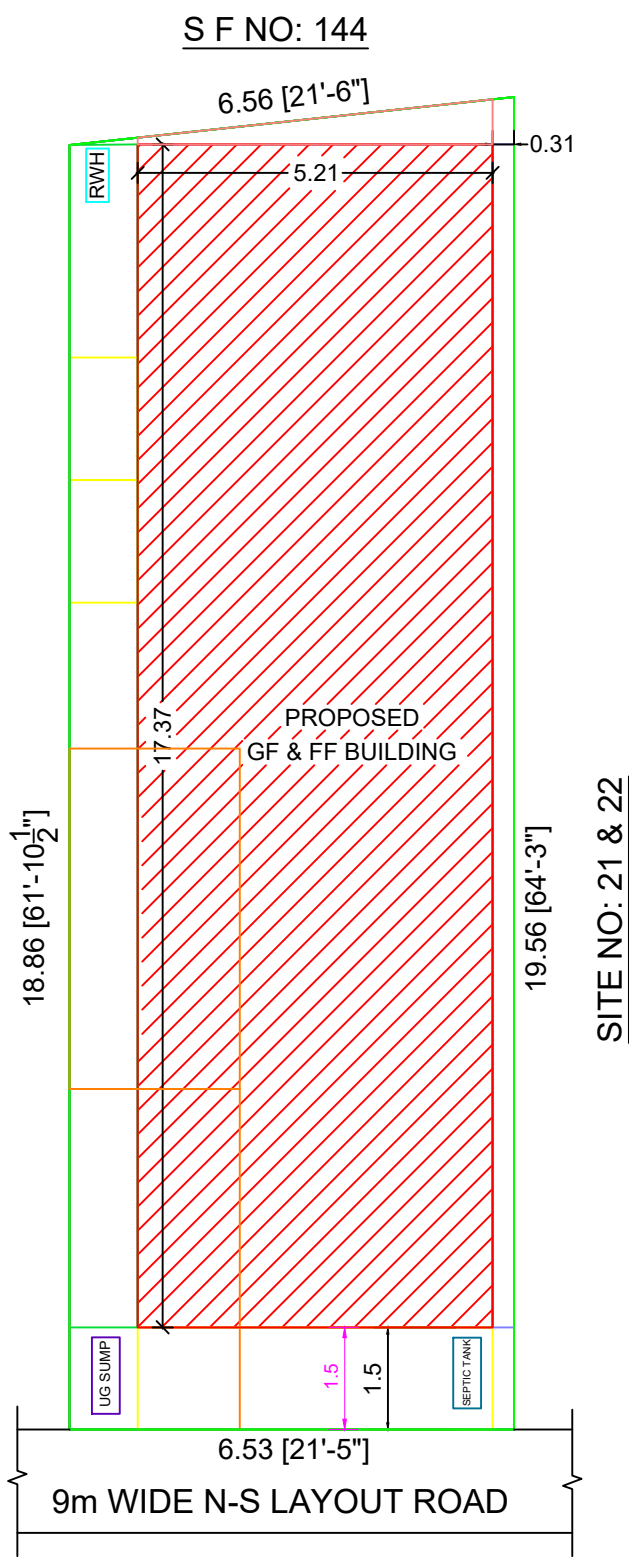
SITE PLAN
