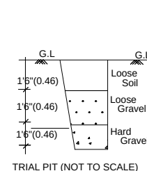
TRIAL PIT (NOT TO SCALE)
