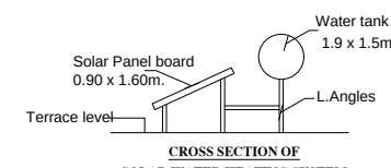
CROSS SECTION OF SOLAR WATER HEATING SYSTEM
