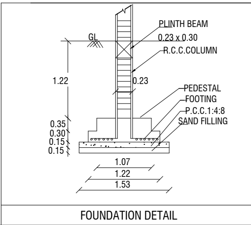
FOUNDATION DETAIL
