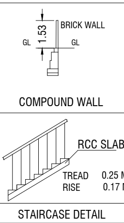
STAIRCASE DETAIL
