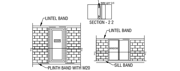
FIGURE 2: REINFORCEMENT AND BENDING DETAILS OF SEISMIC BANDS
