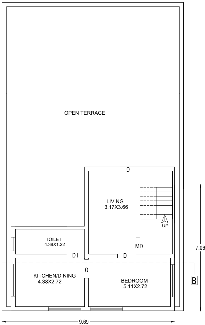
PROPOSED TYPICAL FIRST AND SECOND FLOOR PLAN
