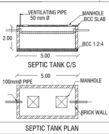
SEPTIC TANK PLAN
