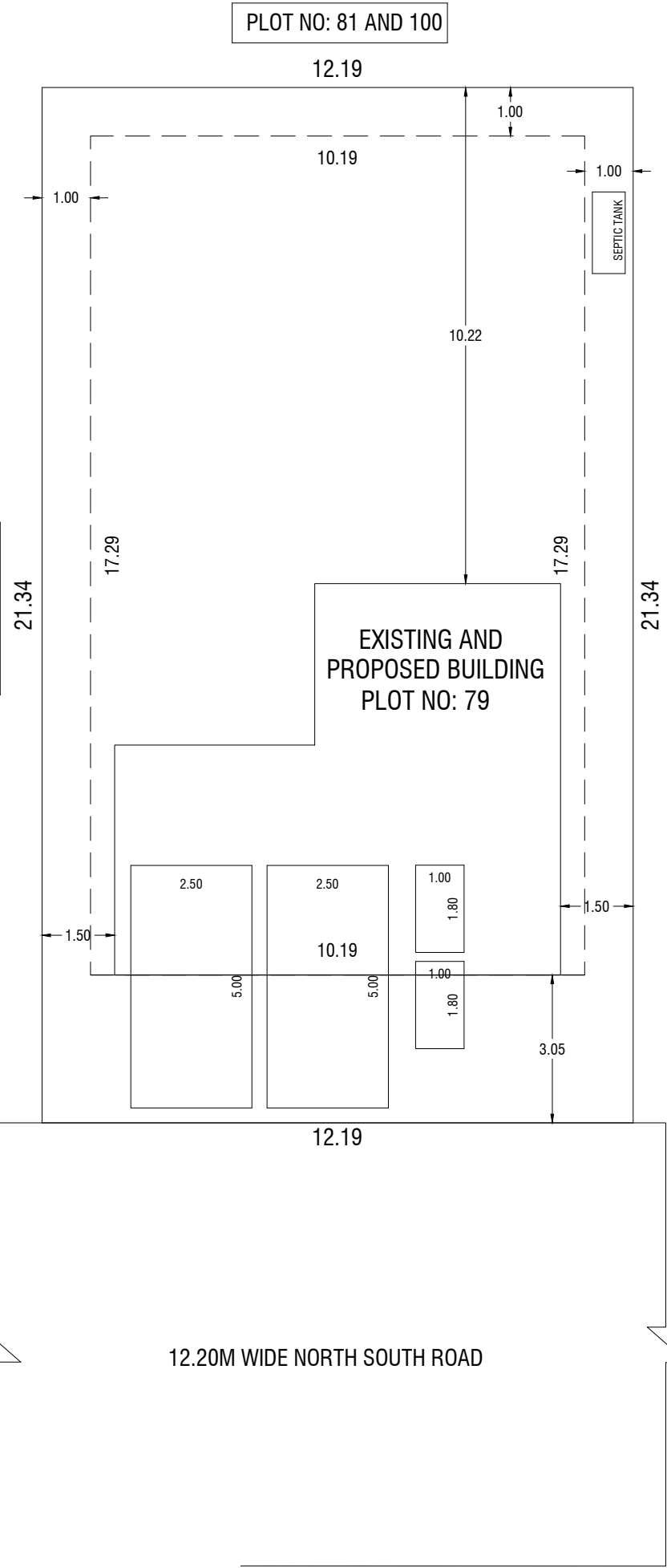
SITE PLAN
