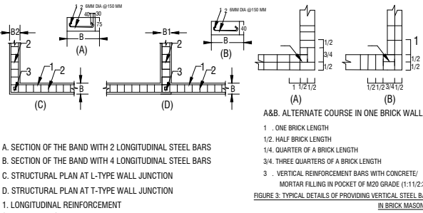
FIGURE 2: REINFORCEMENT AND BENDING DETAILS OF SEISMIC BANDS
