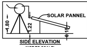
SIDE ELEVATION (NOT TO SCALE)
