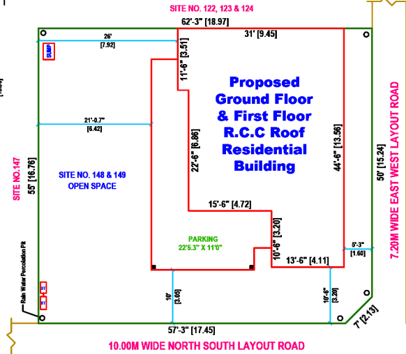
SITE PLAN (SCALE 1" : 8' 0")
