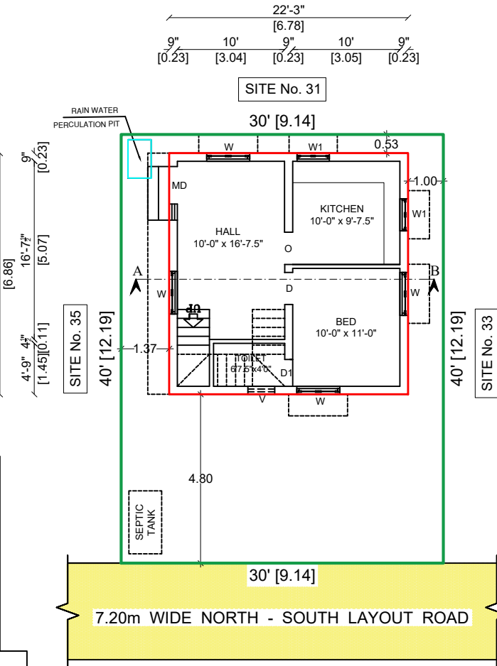
SITE CUM GROUND FLOOR PLAN
