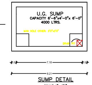
SUMP DETAIL SCALE : 1" = 4'-0"
