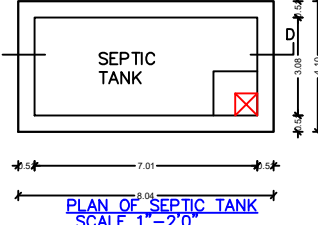
PLAN OF SEPTIC TANK SCALE 1"=2'-0"
