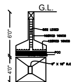
FOUNDATION DETAILS (NOT TO SCALE)
