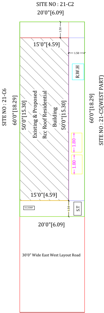
SITE PLAN
