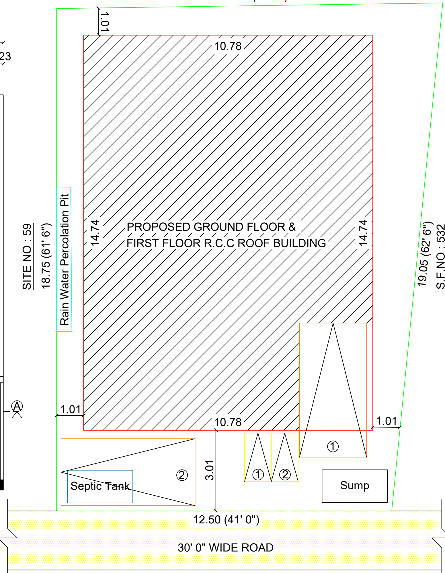
SITE PLAN
