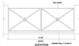
COMPOUND WALL DETAIL SCALE = 1 : 50
