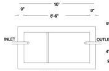
PLAN DETAILS OF SEPTIC TANK
